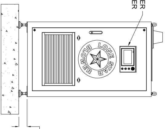
VIEW "C" (FRONT SIDE)
